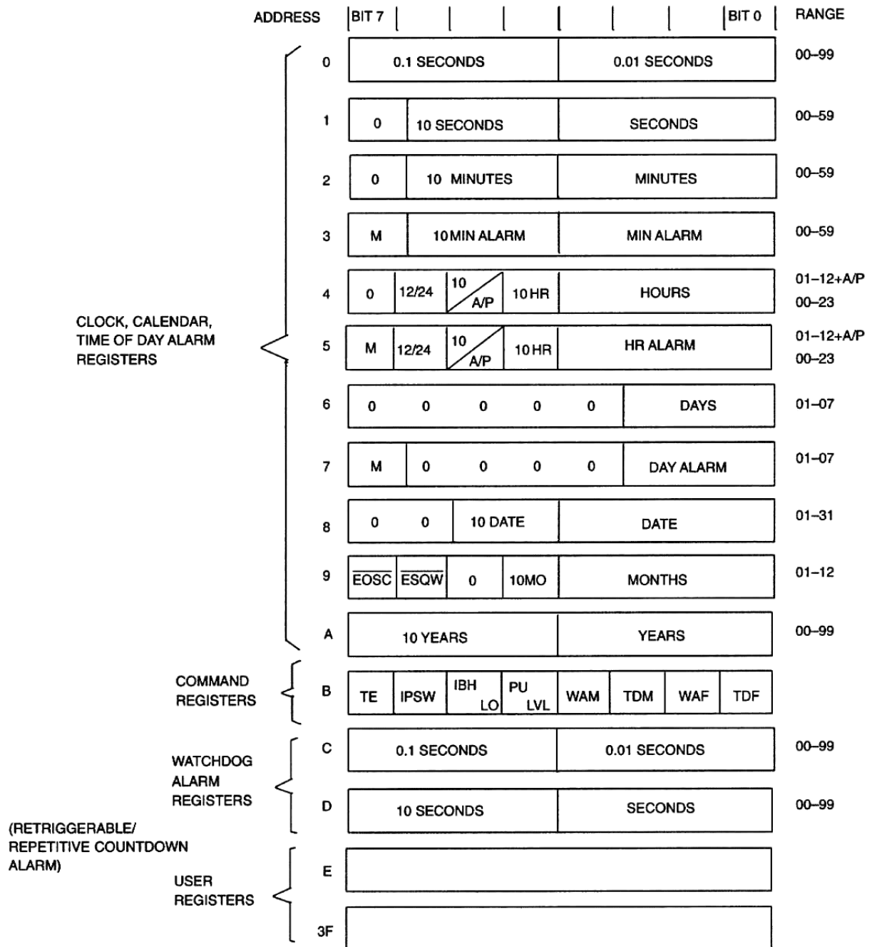
DS1286 WATCHDOG TIMEKEEPER REGISTERS Figure 2
